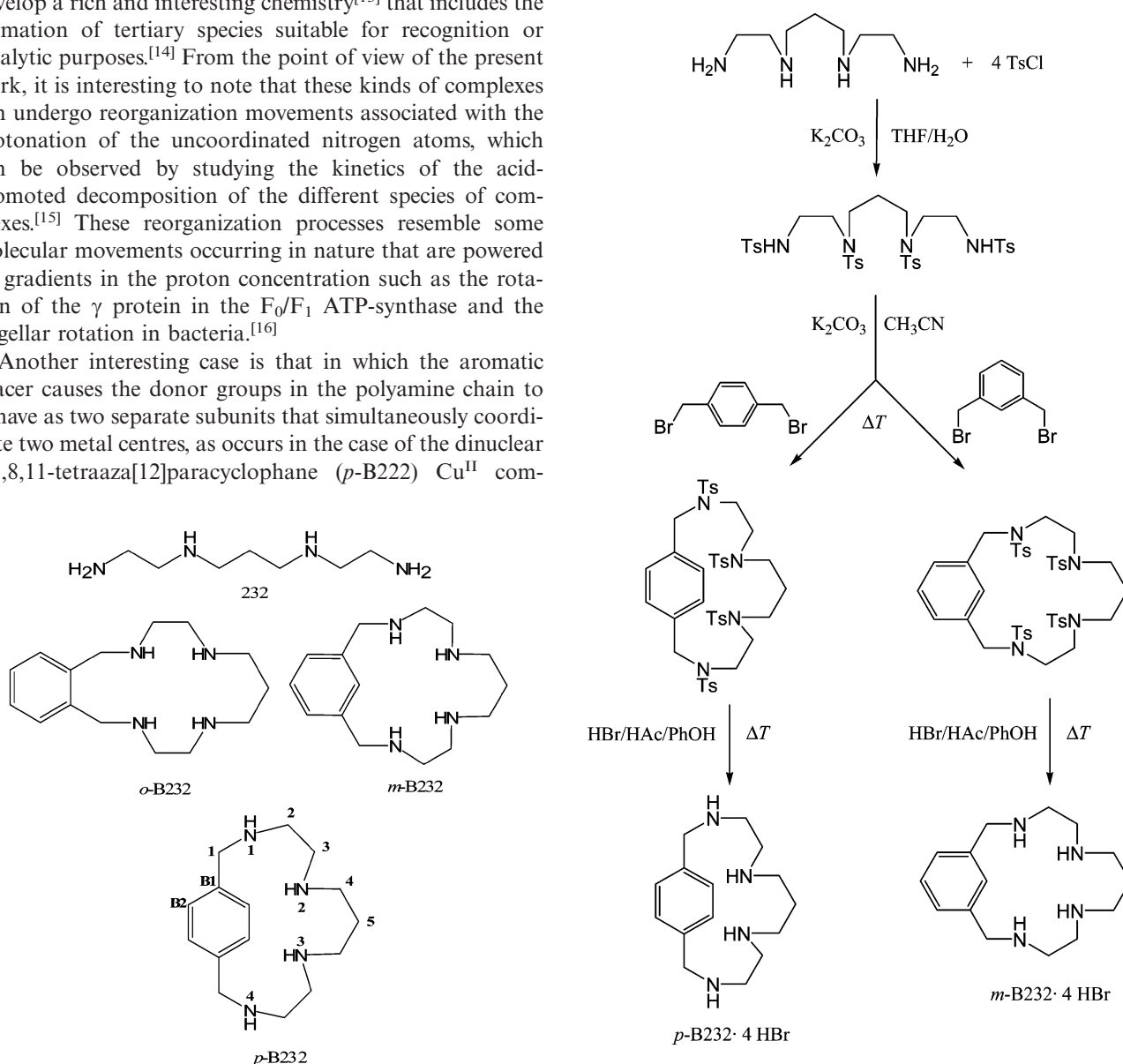
Figure 1. Synthetic pathway for the synthesis of the m -B232 and p -B232 cyclophanes.
