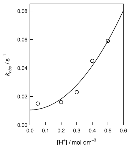
Figure 7. Plot of the acid concentration dependence of the observed rate constant for the acid-promoted decomposition of the Cu II complexes with the o -B232 ligand.
