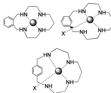
Figure 3. Schematic representation of copper coordination with m -B232, o -B232 and p -B232.
