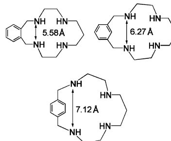
Figure 2. Estimated size of the macrocyclic cavity in the o -B232, m -B232 and p -B232 cyclophanes as calculated with molecular modeling.
