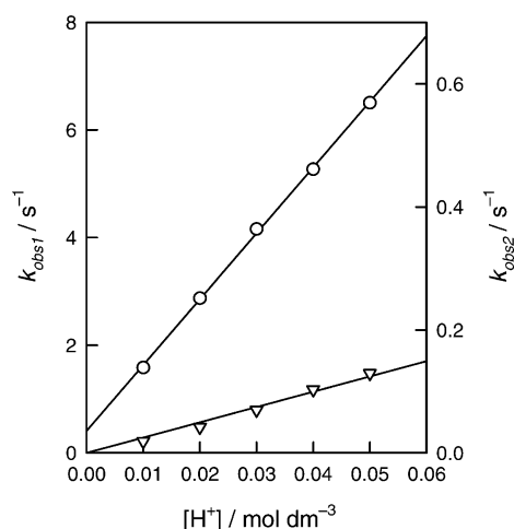
Figure 8. Plot of the acid concentration dependence of the observed rate constants for the acid-promoted decomposition of the mononuclear \text{Cu}^{\text{II}} complexes with the m\text{-B232} ligand. The circles and the triangles correspond to the k_{1\text{obs}} and k_{2\text{obs}} , respectively.
