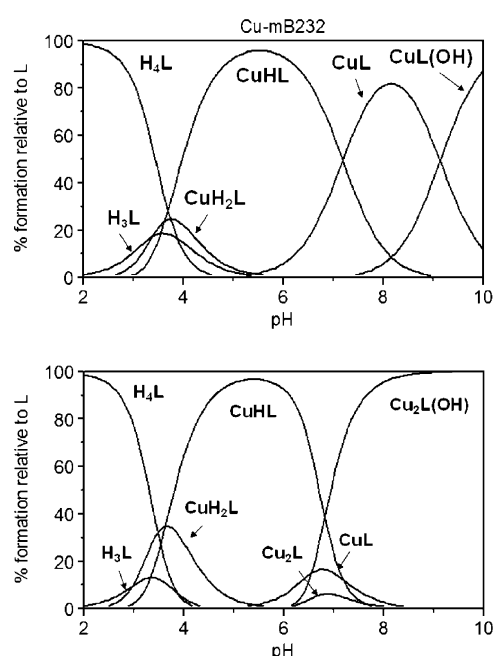
Figure 4. Species distribution curves for the formation of Cu II complexes with the m -B232 cyclophane. The curves were obtained using [L] = 1.0 \times 10^{-3} mol dm -3 and Cu II in 1:1 (top) or 2:1 (bottom) molar ratios.
