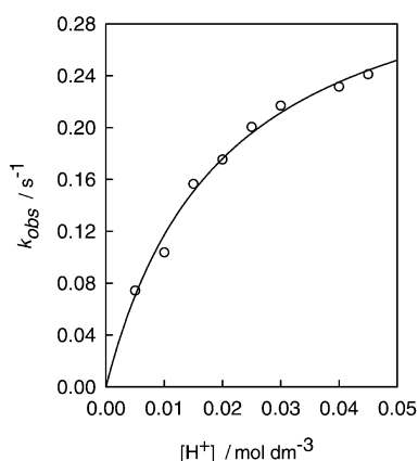
Figure 6. Plot of the acid concentration dependence of the observed rate constant for the acid-promoted decomposition of the \text{Cu}^{\text{II}} complexes with the 232 ligand.
