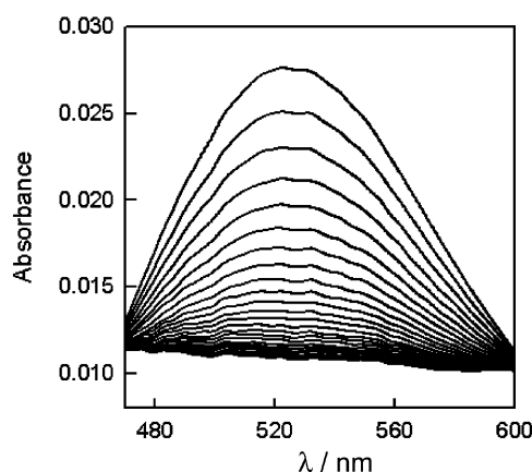
Figure 5. Typical spectral changes observed during the acid-promoted decomposition of the \text{Cu}(232)^{2+} complex. Plotted spectra were recorded at 0.825 s intervals and show the complete disappearance of the \text{Cu}(232)^{2+} absorbance centred at ca. 530 nm.
